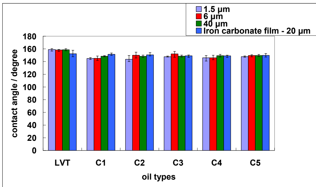
Figure 17 Equilibrium oil-in-water contact angle on different steel surface for different oils
