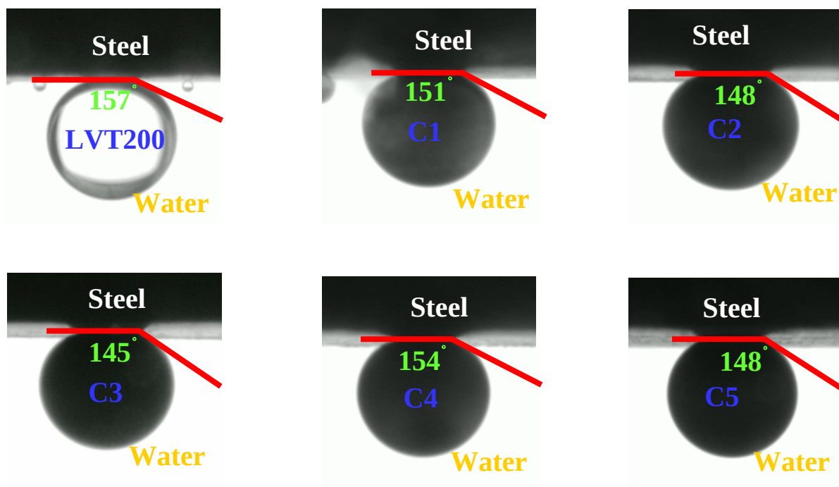
Figure 18 Typical images of different oil droplets on 6 \mu\text{m} steel surface
