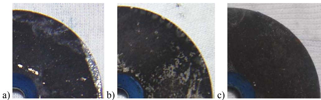
Figure 34. Experiment 3: X65(2) coupons exposed for (a) 10, (b) 15, and (c) 25 days. (60°C, 0.77 MPa CO 2 , pH 6, 12 ± 5ppm H 2 S).
