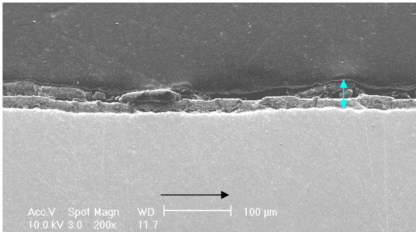
Figure 24. Experiment 3: Cross Section of small UNS C1018 WL coupon from multiphase flow. SEM at 200X magnification shows a 30 \mu m total film thickness. (60°C, 0.77 MPa CO 2 , pH 6, H 2 S gas phase concentration = 120 \pm 10 ppm, 25 day exposure).
