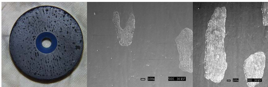
Figure 5. Experiment 1: X65(2), 10 day exposure to multiphase flow, examples of degradation of the film by fluid flow. Flow is in the “upward” direction of the picture. (60°C, 0.77 MPa CO 2 , pH 6, Vsg = 3m/s, Vsl = 1m/s, H 2 S gas phase concentration = 25 ± 10 ppm)
