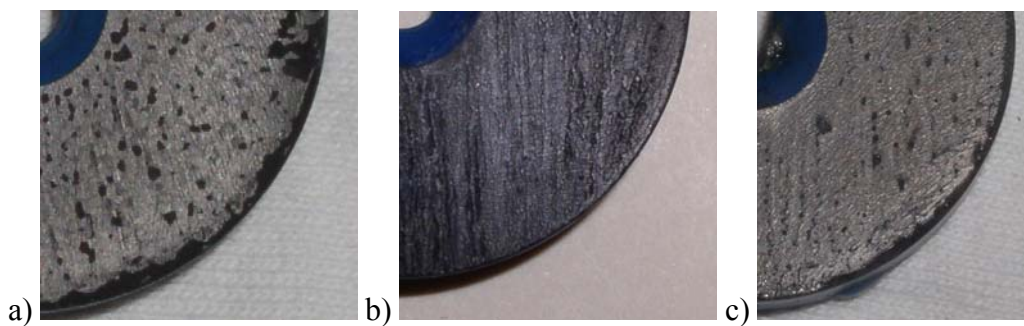
Figure 32. Experiment 1: X65(2) coupons exposed for (a) 10, (b) 20, and (c) 30 days. (60°C, 0.77 MPa CO 2 , pH 6, 25 ± 10ppm H 2 S).
