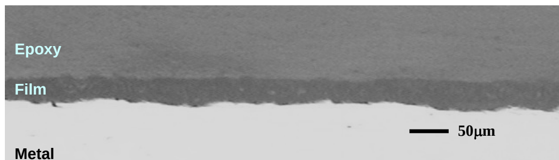
Figure 18. Experiment 2: Cross section of X65(2) WL coupon from multiphase flow exposure shows a 28 to 30 μm film thickness. (100X metallurgical microscope, 60°C, 0.77 MPa CO 2 , pH 6, 12 ± 5ppm H 2 S, 30 day exposure).
