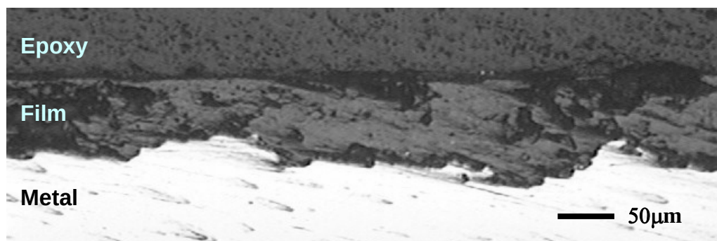
Figure 7. Experiment 1: X65(2), 30 day exposure to single phase flow, 52μm to 103 μm film thickness. (100X metallurgical microscope, 60°C, 0.77 MPa CO 2 , pH 6, Vsg = 3m/s, Vsl = 1m/s, H 2 S gas phase concentration = 25 ± 10 ppm)
