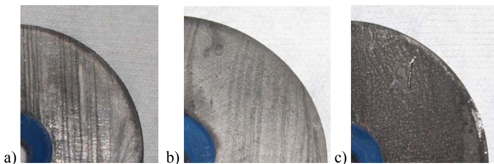
Figure 33. Experiment 2: X65(2) coupons exposed for (a) 10, (b) 20, and (c) 30 days. (60°C, 0.77 MPa CO 2 , pH 6, 12 ± 5ppm H 2 S).
