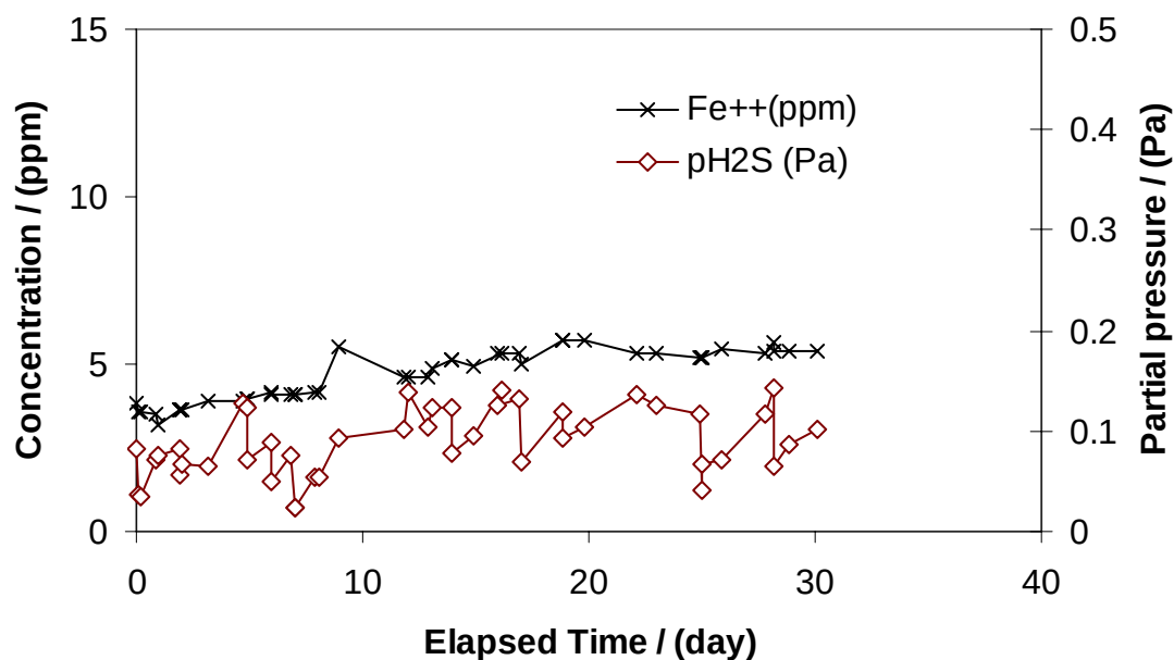
Figure 14. Experiment 2: Variations of iron and hydrogen sulfide concentrations with time. (60°C, 0.77 MPa CO 2 , pH 6, 12 ± 5ppm H 2 S).
