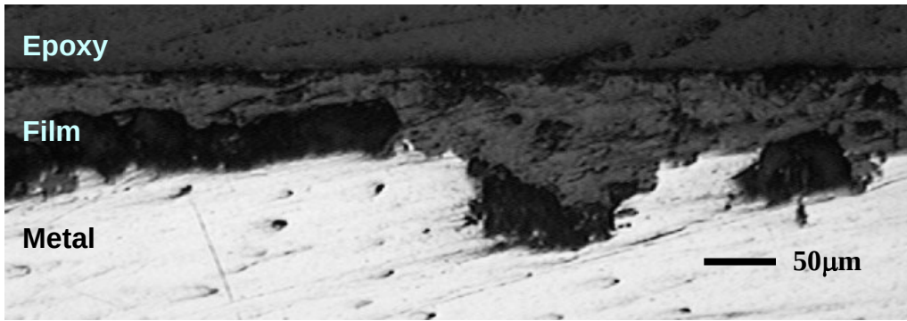
Figure 8. Experiment 1: X65(2), 30 day exposure to single phase flow, 60 to 125 μm film thickness, showing pitting. (100X metallurgical microscope, 60°C, 0.77 MPa CO 2 , pH 6, V sg = 3m/s, V sl = 1m/s, H 2 S gas phase concentration = 25 ± 10 ppm).
