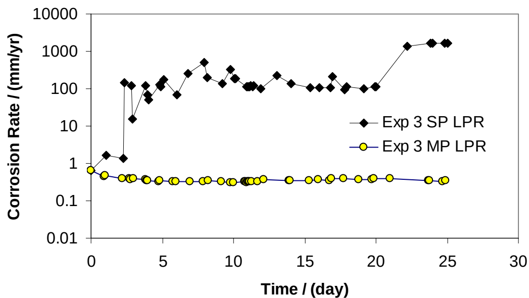
Figure 23. Experiment 3: Measured values for single phase LPR and multiphase LPR corrosion rate with time. Single phase LPR measurements affected by conductive FeS films (60°C, 0.77 MPa CO 2 , pH 6, H 2 S gas phase concentration = 120 ± 10 ppm)
