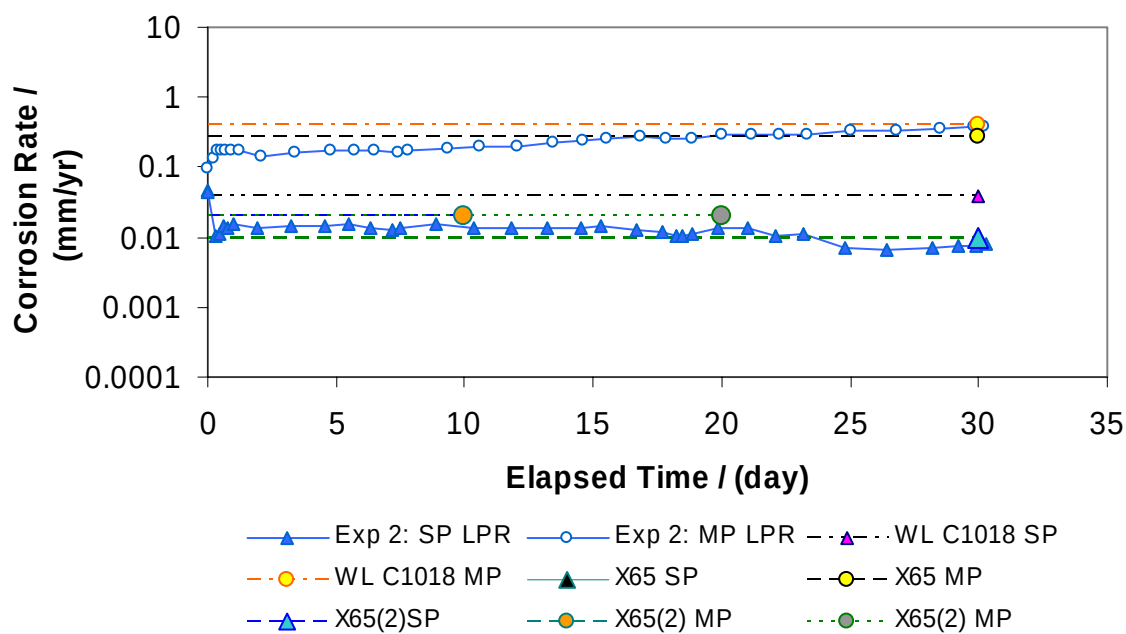
Figure 16. Experiment 2: Corrosion Rates measured by LPR and single C1018 WL values. (60°C, 0.77 MPa CO 2 , pH 6, 12 ± 5ppm H 2 S).
