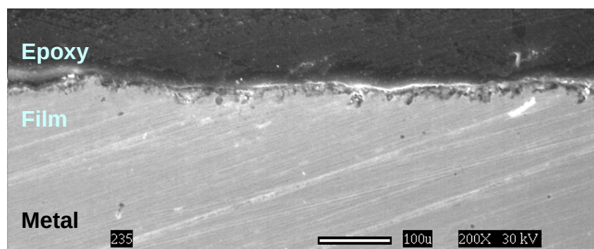
Figure 19. Experiment 2: Cross section of UNS C1018 WL coupon from multiphase flow exposure shows a 15 to 30 μm film thickness. (60°C, 0.77 MPa CO 2 , pH 6, 12 ± 5ppm H 2 S, 30 day exposure).
