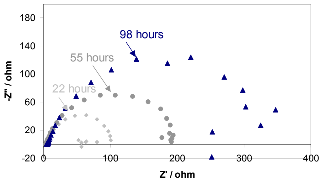
Figure 20. Nyquist plot for single phase flow with time in 100 ppm \text{H}_2\text{S} in pH 6 single phase solution. (0.79 MPa \text{CO}_2 , 60°C, 1% NaCl, and V_{sl} = 1.0\text{m/s} )
