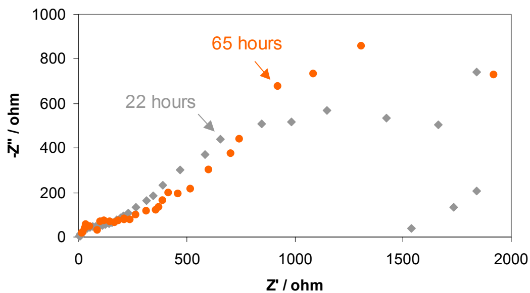
Figure 15. Nyquist plot for single phase flow with time in 100 ppm \text{H}_2\text{S} in pH 5 single phase solution. (0.79 MPa \text{CO}_2 , 60°C, 1% NaCl, and V_{sl} = 1.0\text{m/s} )
