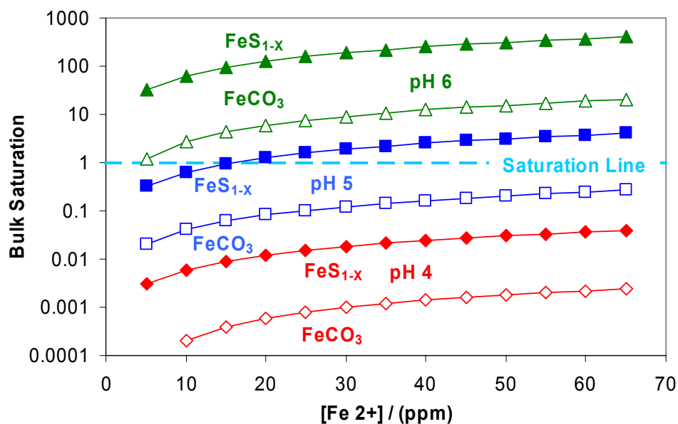
Figure 2. Theoretical calculation of bulk solution saturation values at test conditions. (0.79 MPa \text{CO}_2 , 60°C, 100 ppm \text{H}_2\text{S} , 1% NaCl)
