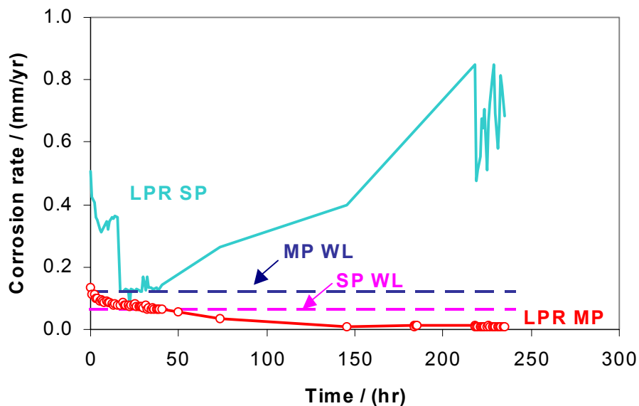
Figure 31. Corrosion rates measured by LPR and WL exposed to 25 ppm \text{H}_2\text{S} in pH 6.0 solution. (0.77 MPa \text{CO}_2 , 60°C, 1% NaCl, V_{\text{sl}} = 1.0\text{m/s} )
