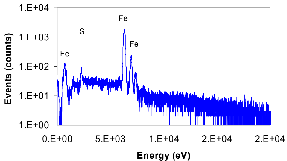
Figure 19. EDS of coupon surface after exposure to 100 ppm \text{H}_2\text{S} in pH 5 solution Single phase. (0.79 MPa \text{CO}_2 , 60°C, 1% NaCl, V_{sl} = 1.0\text{m/s} , 96 hrs.)
