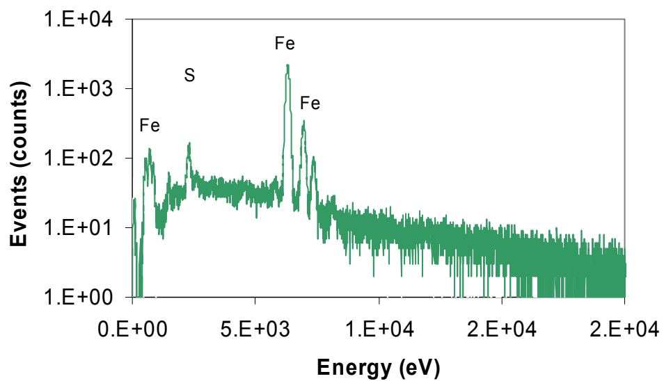
Figure 14. EDS of coupon surface after exposure to 100 ppm \text{H}_2\text{S} in pH 5 solution Single phase. (0.79 MPa \text{CO}_2 , 60°C, 1% NaCl, V_{sl} = 1.0\text{m/s} , 96 hrs.)
