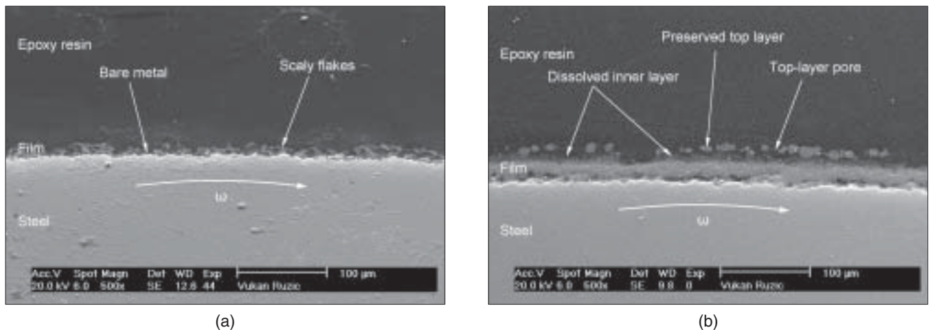
FIGURE 2. Typical cross section of: (a) low-pH – low-velocity (pH 3 – 200 rpm) and (b) high-pH – high-velocity (pH 5.5 – 10,000 rpm) \text{FeCO}_3 film residual at the end of dissolution process (mag. 500X).
