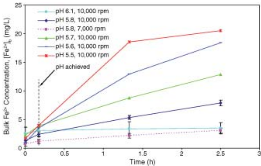
FIGURE 19. Mean measured \text{Fe}^{2+} concentration in bulk solution during the film dissolution in the pH 5.5 to 6.1 range (bars represent standard deviation of the mean, i.e., standard error).
