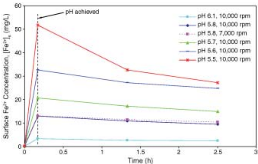
FIGURE 20. Predicted \text{Fe}^{2+} concentration at the film-solution interface during the film dissolution process calculated for saturated condition ( S = 1 ) given the measured pH.
