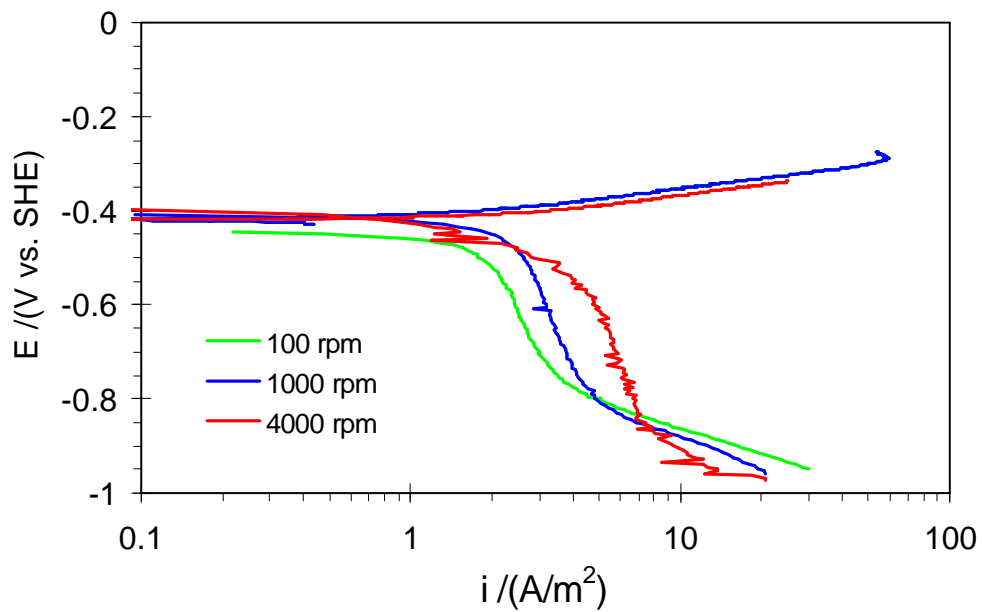
Figure 3. Potentiodynamic sweep conducted in a CO_2 solution at pH 4, t=22\text{ }^\circ\text{C} , 3% NaCl, using a rotating cylinder electrode d=1\text{ cm} .
