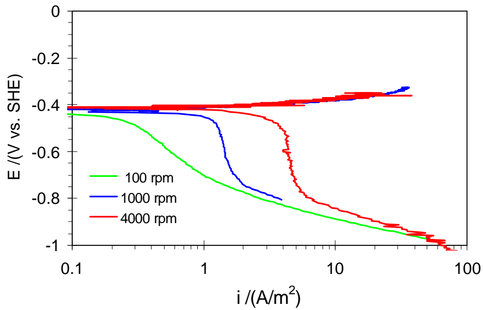
Figure 2. Potentiodynamic sweep conducted in HCl solution at pH 4 purged with N_2 , t=22\text{ }^\circ\text{C} , 3% NaCl, using a rotating cylinder electrode d=1\text{ cm} .
