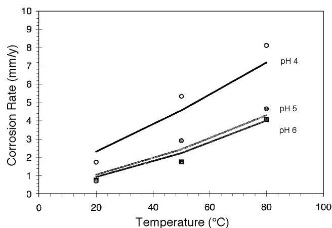
FIGURE 17. Comparison of the model predictions with results from independent glass loop experiments with X-65 steel in water + 1 % NaCl at v = 2 m/s (6.56 ft/s), \tau = 12 Pa, P_{\text{CO}_2} = 1 bar (100 kPa), and Re = 30,000 .
