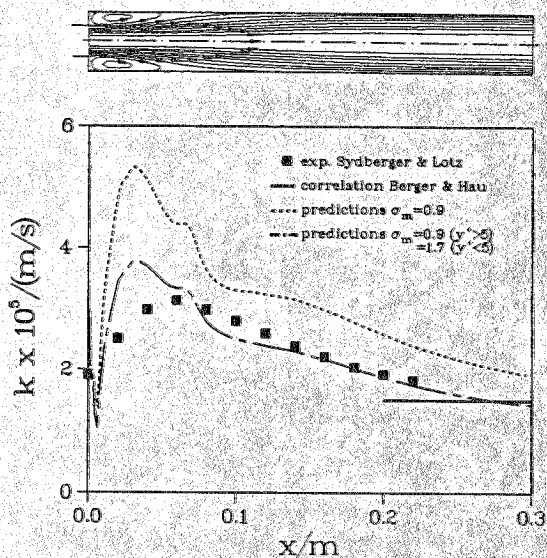
FIG. 2. Predicted flow streamlines and measurements and predictions for the mass transfer coefficients. Water flow through a sudden pipe expansion; d_{in} = 20.0 mm; d_{out} = 40.0 mm; v_{in} = 1.71 m s -1 ; v_{out} = 0.42 m s -1 ; Re_{out} = 2.1 \times 10^4 .
