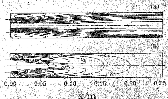
FIG. 1. Predictions for (a) the flow streamlines and (b) corresponding turbulence kinetic energy field. Water flow through a sudden pipe expansion; d_{in} = 20.0 \text{ mm} ; d_{out} = 40.0 \text{ mm} ; v_{in} = 1.71 \text{ m s}^{-1} ; v_{out} = 0.42 \text{ m s}^{-1} ; Re_{in} =
