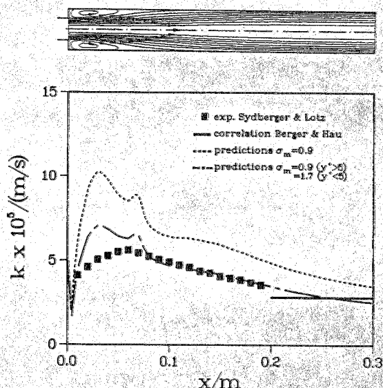
FIG. 3. Predicted flow streamlines and measurements and predictions for the mass transfer coefficients. Water flow through a sudden pipe expansion; d_{in} = 20.0 mm; d_{out} = 40.0 mm; v_{in} = 3.38 m s -1 ; v_{out} = 0.84 m s -1 ; Re_{out} = 10.45 \times 10^4 .
